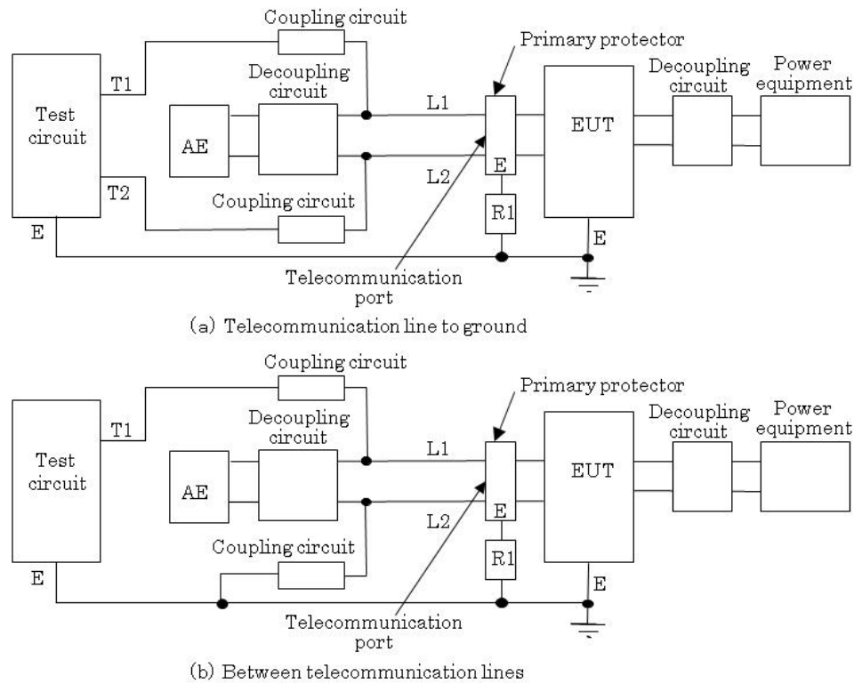
Figure 3-4 Injection circuit for lightning surge test (telecommunication port)
