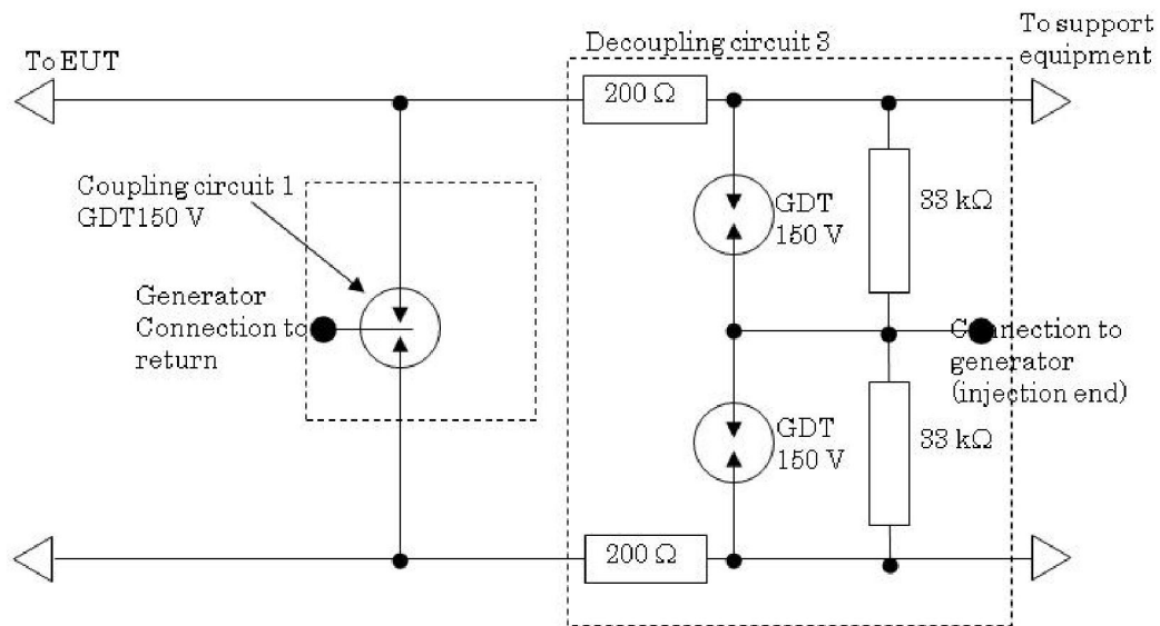
Figure 3-11 Example circuit for test port used in the POTS port surge test (ITU-T K.Imp44 Guide on the Use of the Overvoltage Resistibility Recommendations Fig. 61)
