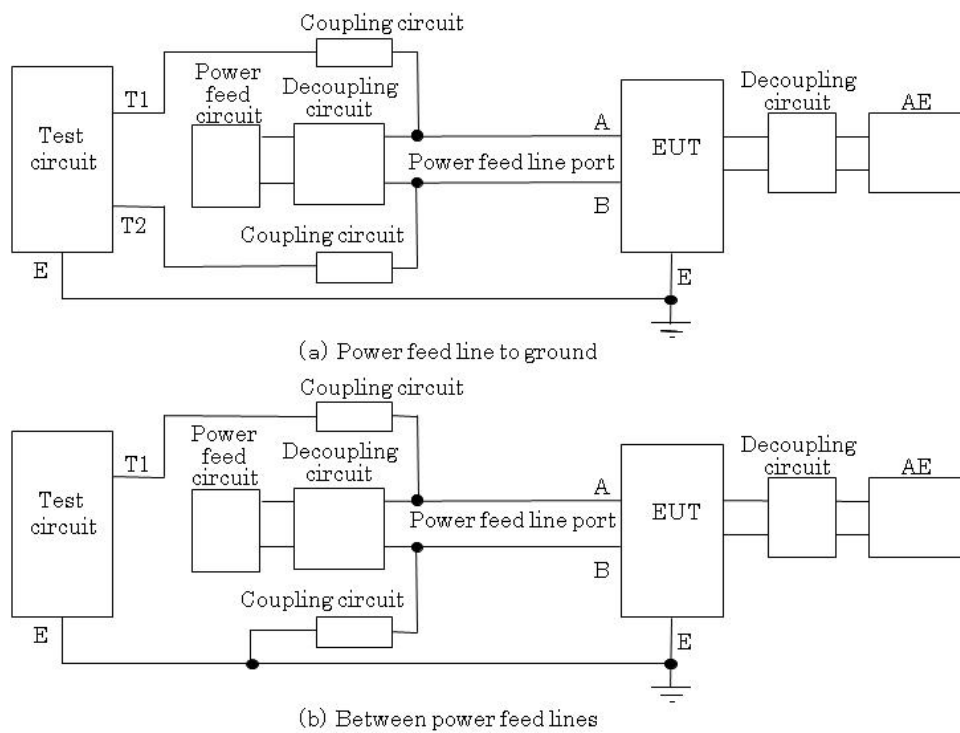
Figure 3-6 Injection circuit for lightning surge test (power feed port, outdoor exposure assumed)
