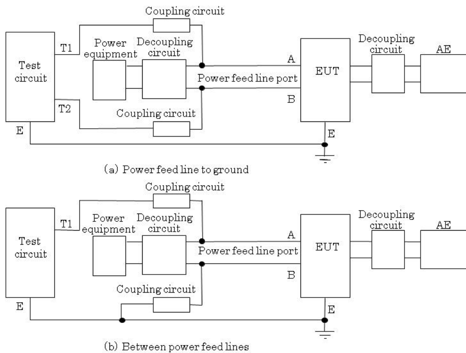
Figure 2-3 Injection circuit for the contact test (outdoor exposed power feed line)
