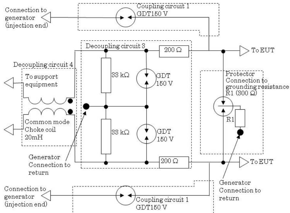
Figure 3–10 Example circuit for test port used in the POTS port surge test (ITU–T K.Imp44 Guide on the Use of the Overvoltage Resistibility Recommendations Fig. 59)
