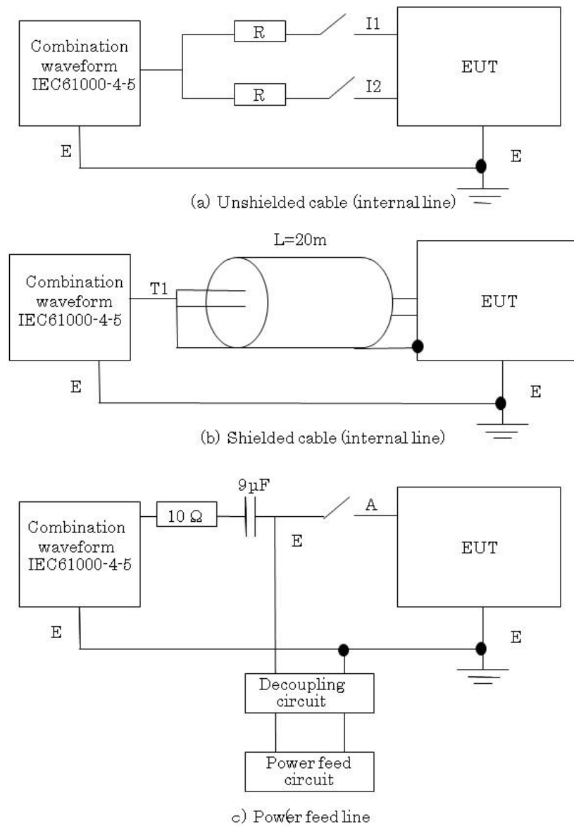
Figure 3-8 Injection circuit for lightning surge test (internal port and power feed port for telecommunication center)
