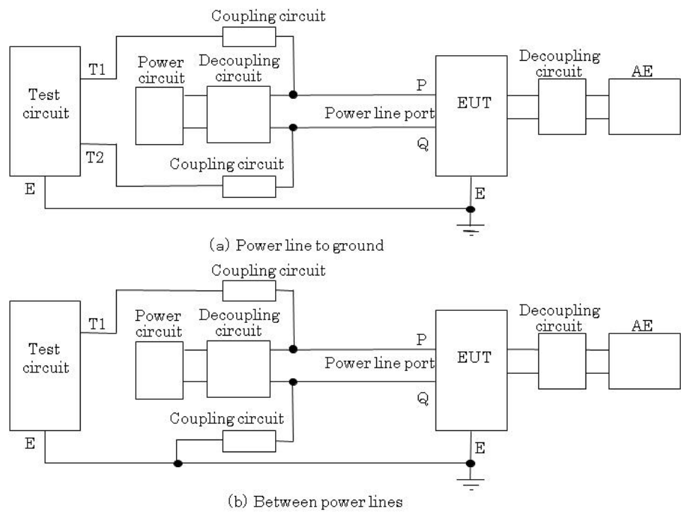
Figure 3-5 Injection circuit for lightning surge test (commercial power port)
